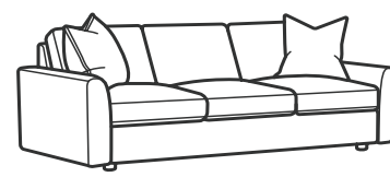
-31 SOFA 33H 87W 39D 19SH 77SW 24SD 25AH
