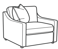
-10 CHAIR 33H 37W 39D 19SH 30SW 24SD 22AH
